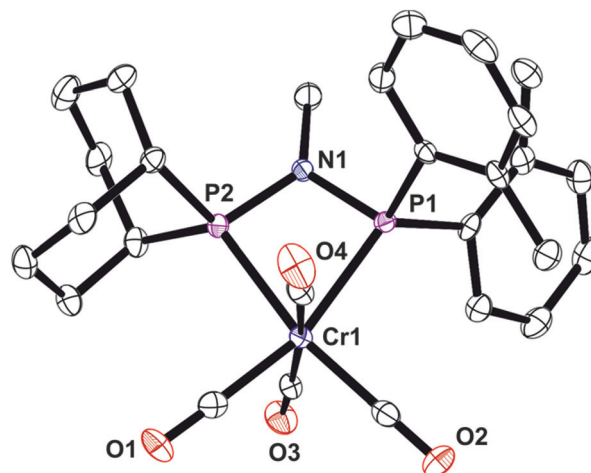
Fig. 9 Crystal structure of [\text{Cr}(\text{CO})_4(L_g)] ( 8 ). All hydrogen atoms have been omitted for clarity. Selected bond lengths ( \text{\AA} ) and angles ( ^\circ ): \text{Cr}(1)-\text{P}(1) 2.3477(6), \text{Cr}(1)-\text{P}(2) 2.3669(6), \text{P}(1)-\text{N}(1) 1.7146(17), \text{P}(2)-\text{N}(1) 1.7035(17), \text{P}(1)-\text{Cr}(1)-\text{P}(2) 68.04(4), \text{P}(2)-\text{N}(1)-\text{P}(1) 101.01(9), \text{N}(1)-\text{P}(1)-\text{Cr}(1) 94.67(6), \text{N}(1)-\text{P}(2)-\text{Cr}(1) 94.29(6), \text{C}(16)-\text{P}(1)-\text{C}(13) 95.66(10), \text{C}(7)-\text{P}(2)-\text{C}(4) 105.17(9).
