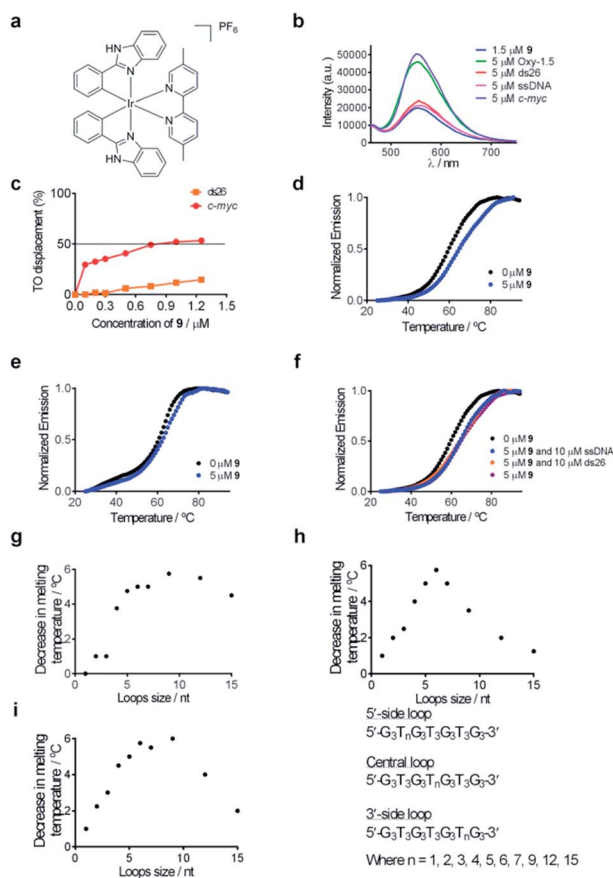
Fig. 2 (a) Chemical structure of complex 9 . (b) Emission spectrum of complex 9 (1.5 \mu\text{M} ) in the presence of 5 \mu\text{M} of ssDNA, ds26 or various G-quadruplexes. (c) G4-FID titration curves of complex 9 with duplex (ds26) or G-quadruplex ( c-myc ) DNA. (d) Melting profile of F21T G-quadruplex DNA (0.2 \mu\text{M} ) in the absence and presence of 9 (5 \mu\text{M} ). (e) Melting profile of F10T dsDNA (0.2 \mu\text{M} ) in the absence and presence of 9 (5 \mu\text{M} ). (f) Melting profile of F21T G-quadruplex DNA (0.2 \mu\text{M} ) in the absence and presence of 9 (5 \mu\text{M} ) and ds26 (10 \mu\text{M} ) or ssDNA (10 \mu\text{M} ). (g–i) Competitive FRET-melting assay results for complex 9 in the presence of G-quadruplexes with different loop lengths as the competitor. The decrease in melting temperature is shown as a function of loop size.
