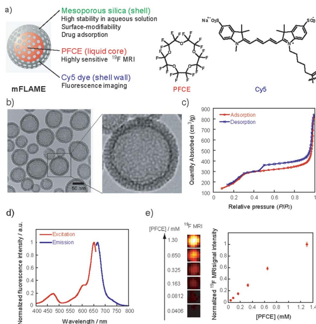
Fig. 1 (a) The components of mFLAME. (b) Transmission electron microscopy (TEM) image of mFLAME. (c) \text{N}_2 adsorption/desorption isotherms of mFLAME. (d) Excitation and fluorescence spectra of mFLAME in phosphate buffered saline (pH 7.4). (e) (Left) ^{19}\text{F} MRI of mFLAME in phosphate buffered saline (500 \mu\text{L} ); (right) plot of normalized ^{19}\text{F} MRI signal intensity versus PFCE concentration.
