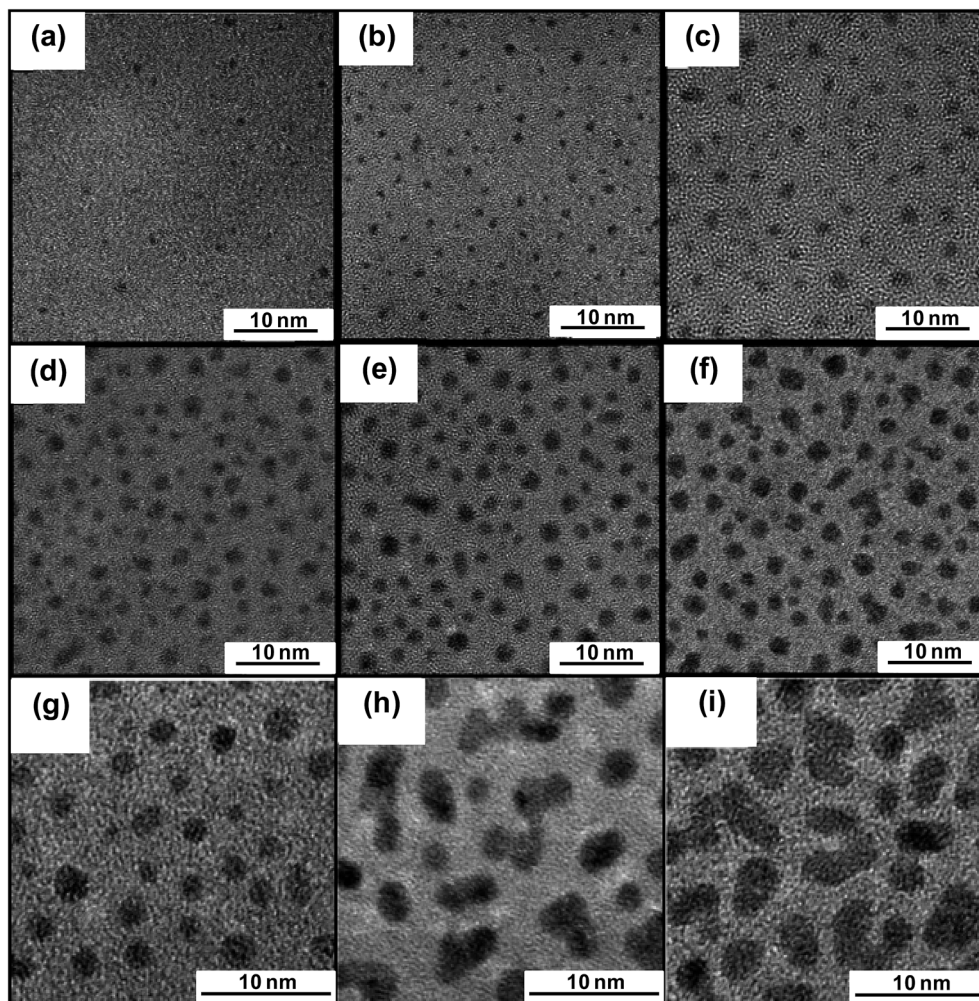
Fig. 5 High resolution transmission electron microscopy images of Pt NPs synthesized by sputtering process. (a)–(f) Pt NPs grown at constant target angle of 23.8° but varied growth time of (a) 5 s, (b) 10 s, (c) 20 s, (d) 30 s, (e) 45 s and (f) 55 s. (g)–(i) Pt NPs grown at constant growth time of 2 min but varied target angle of (g) 16.2°, (h) 23.8° and (i) 38.8°. Reproduced with permission from ref. 85.
