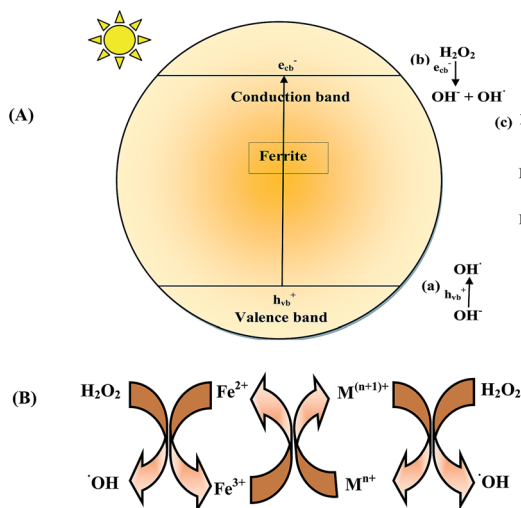
Fig. 12 (A) Mechanism of generation of a hydroxyl radical ( \text{OH}^{\cdot} ) in the presence of a ferrite/ \text{H}_2\text{O}_2 /light system. (B) General mechanism of electron transfer occurring in ferrite.
