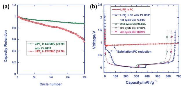
Fig. 20 (a) Cycling performance of LiNi 0.5 Mn 1.5 O 4 in the reference and HFIP-containing electrolytes. Percent capacity retention is shown for easy comparison. (b) Voltage profiles of the graphite anodes in the PC-based electrolyte with and without 1% HFIP additive. Reproduced with permission. 96
