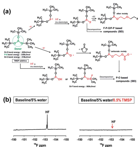
Fig. 19 (a) Proposed mechanisms for electrochemical oxidative decomposition of TMSP and for the unique function of TMSP scavenging HF from the electrolyte. (b) 19 F NMR spectra of the electrolyte with and without TMSP. Reproduced with permission. 92
