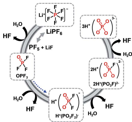
Fig. 18 Hydrolysis reactions of LiPF 6 salt in the presence of trace water in the cell.
