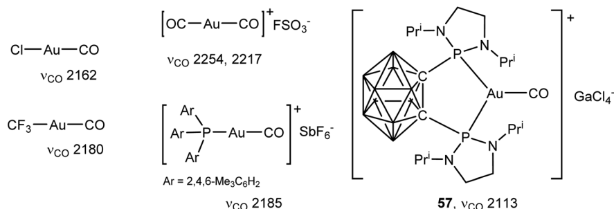
Scheme 27 Representative types of Au(I) CO complexes, with \nu_{\text{CO}} stretching frequencies (cm −1 ). 128,129,133,138
