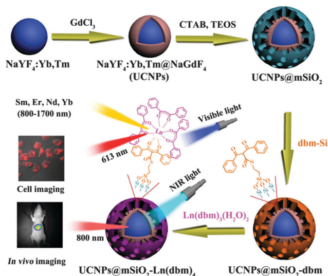
Fig. 13 Schematic of the preparation and structure of multifunctional mesoporous NPs containing both upconversion and magnetic nanoporphors (with an architecture of the type NaYF 4 :Yb,Tm@NaGdF 4 ) and covered with a conventional luminescent lanthanide complex (Ln-db m ) for use in upconversion and downconversion luminescence imaging and as T 1 -weighed MRI contrast agents. From ref. 257 © RSC.
