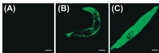
Fig. 33 Top: schematic representation of the \text{Cu}(\text{II}) displacement approach to sensing cyanide. Middle: structure and displacement reaction of 38-Cu(II) . Bottom: fluorescence images of (A) young adult nematodes previously incubated with 38 then incubated with \text{Cu}(\text{II}) , (B) nematodes previously incubated with 38 and \text{Cu}(\text{II}) then incubated with one equiv. of \text{CN}^- or (C) with ten equiv. of \text{CN}^- . Scale = 50 \mu\text{m} . Image reproduced with permission. 179
