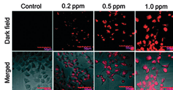
Fig. 35 Structure of DPA functionalised Ir complex 40 . Bottom: images of live HeLa cells in the presence of 40-Cu(II) acquired after treatment with increasing concentrations of \text{NaCN} . Image reproduced with permission. 182
