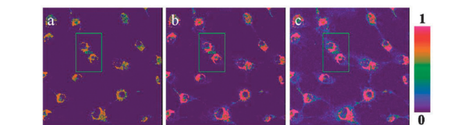
Fig. 52 Top: structure and reaction of HS-Cy with \text{HS}^- . Bottom: confocal fluorescence ratiometric images of endogenous \text{HS}^- in living A549 cells. A549 cells loaded with 5 \text{ mM} HS-Cy for 30 min (a). Cells were pre-stimulated with SNP, then incubated with HS-Cy for 10 min (b) and 20 min (c). Scale = 50 \text{ nm} . Image reproduced with permission. 222
