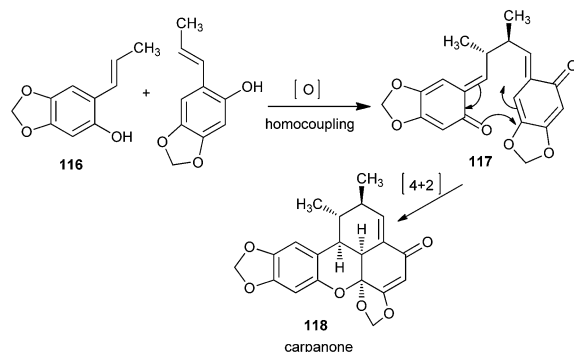
Scheme 26 Synthesis of carpanone via electrocyclicization of o -QM 117 .
