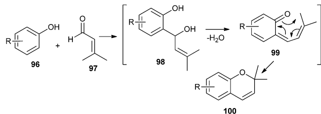
Scheme 22 Synthesis of chromenes via electrocyclicization of o -QMs.
