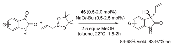
Scheme 31 Allylation of N-protected isatins.
