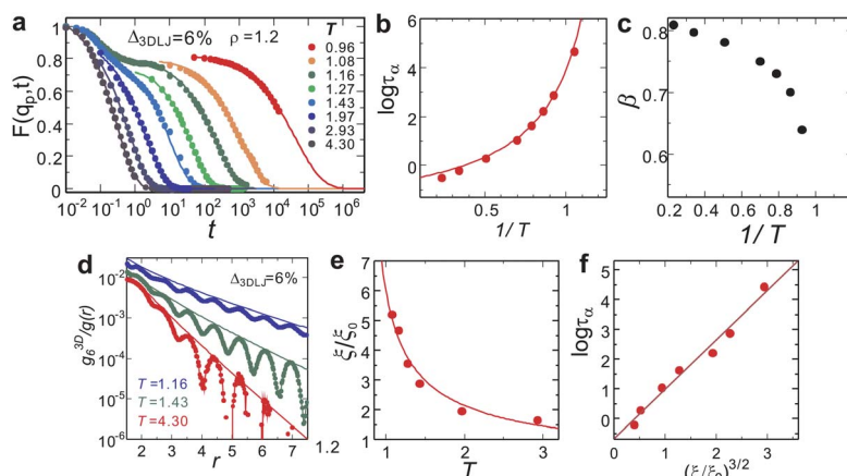
Fig. 27 Dynamical and structural evolution upon cooling in 3D Lennard-Jones system (3DLJ). The density \rho = 1.2 and the polydispersity \Delta_{3DLJ} = 6\% . (a) T -dependence of the intermediate scattering function F(q_p, t) . The solid curve is the stretched exponential function. (b) T -dependence of the structural relaxation time \tau_\alpha . It slows down more than five orders of magnitude upon cooling. The solid curve is the VFT relation. (c) T -dependence of the stretching exponent \beta . (d) The spatial correlation function of the bond orientational order parameter Q_6 , g_6^{3D}(r) . The solid lines are the fittings by the 3D Ornstein–Zernike function. (e) T -dependence of the correlation length \xi . The solid curve is the power law fitting (see text). (f) The relation between \tau_\alpha and \xi .
