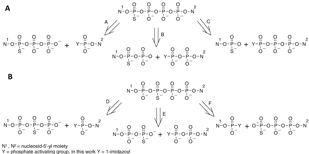
Scheme 2 Possible disconnections of tetraphosphate-bridged thio-modified dinucleotides. (A) Tetrakisphosphates with phosphorothioate modification in the external position. (B) Tetrakisphosphates with phosphorothioate modification in the internal position.
