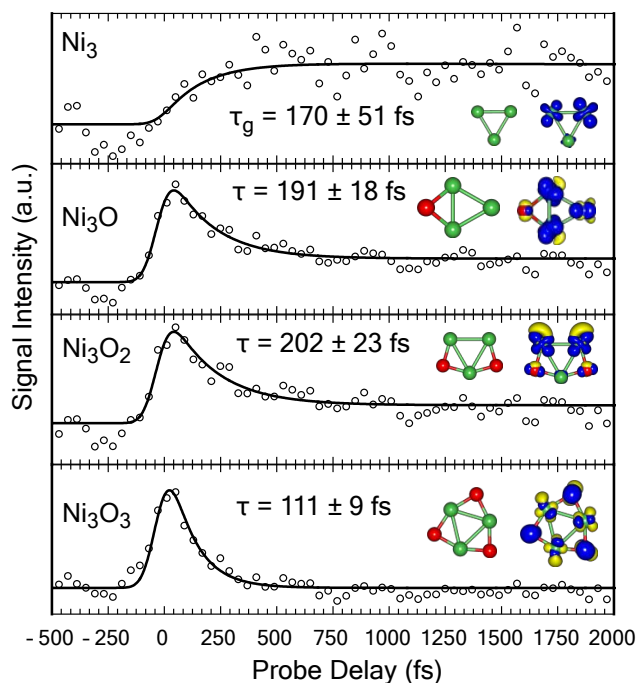
Fig. 5 Transient signal of Ni 3 O x (x < 4) clusters and their structures, similar to Fig. 2.
