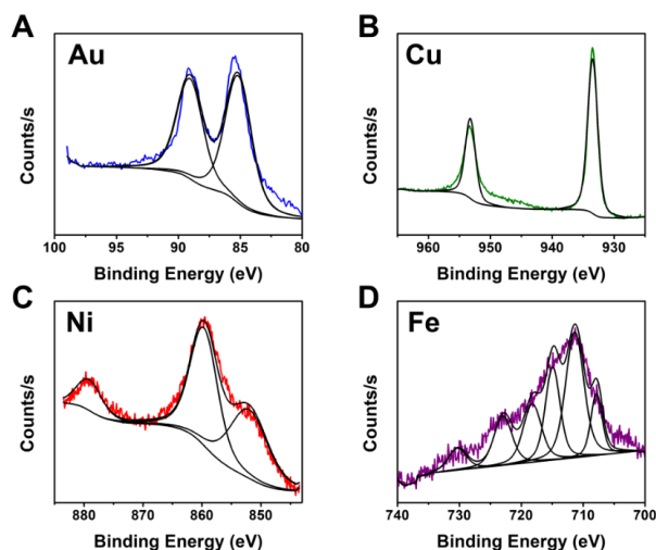
Fig. 7 XPS spectra of Au, Cu, Ni, and Fe NPs. Composition of wells were with 1mM PEGSH and between 1 to 1.4 mM metal.
