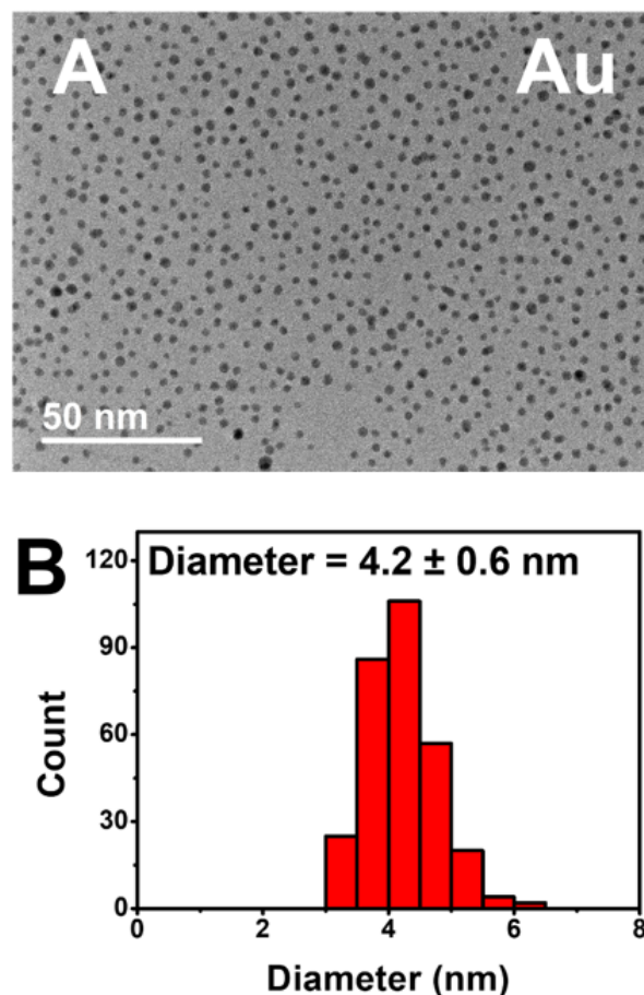
Fig. 6 TEM micrograph and NP size distribution at 1.4 mM metal and 1 mM PEGSH.
