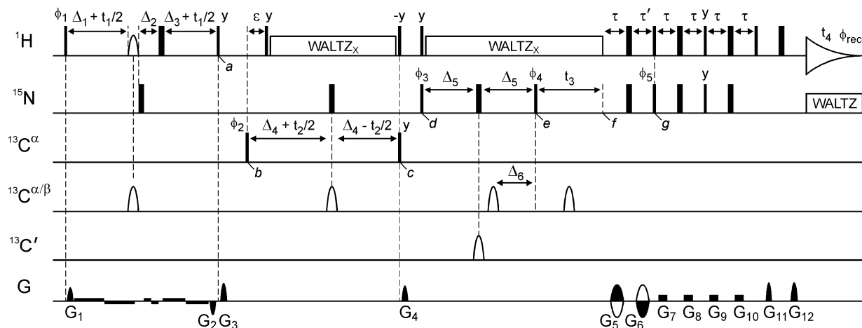
Fig. 1 Pulse scheme of the HACANH[C'] E.COSY experiment. Narrow and wide lines indicate non-selective 90^\circ and 180^\circ pulses, respectively, except for the 90^\circ pulses on ^{13}\text{C}' that have their duration adjusted to have no excitation of ^{13}\text{C}' . ^1\text{H} decoupling ( \gamma_{\text{H}}B_1 = 3.1 kHz; phase x) is applied using the WALTZ16 scheme. 38 The carrier frequencies for ^1\text{H} , ^{15}\text{N} , ^{13}\text{C}^\alpha , ^{13}\text{C}^{\alpha/\beta} and ^{13}\text{C}' are 4.7, 119, 56, 46 and 176 ppm, respectively. The ^1\text{H}^\alpha shaped pulse is of the ReBURP-type and has a duration of 3.5ms. The ^{13}\text{C}' shaped pulse is of the hyperbolic-secant type and has a duration of 2 ms. The ^{13}\text{C}^{\alpha/\beta} shaped pulses are G3-shaped 53 with a duration of 350 \mu\text{s} , except for the pulse during ^{13}\text{C}^\alpha evolution ( t_2 ) which is of the ReBURP-type 54 and has a duration of 420 \mu\text{s} . Note that the durations of all shaped pulses presented here are for measurements at 600 MHz ^1\text{H} frequency; these values scale inversely with field strength and should be adjusted accordingly when experiments are recorded at a field strength that differs from 14.1 T. Delays: \varepsilon = 2.5 ms, \tau = 2.6 ms, \tau' = \tau + t_3(0) , \Delta_1 = 1.7 ms - 0.92 \times P_{\text{rb}}/2 where P_{\text{rb}} is the duration of the ^1\text{H}^\alpha ReBURP pulse and the scaling factor of 0.92 for ^1\text{J}_{\text{C}\alpha\text{H}\alpha} dephasing was measured experimentally for a pair of centered ^1\text{H} ReBURP and ^{13}\text{C} G3 shaped pulses with a duration ratio of 10:1, \Delta_2 = \Delta_1 + \Delta_3 , \Delta_3 = 0.17 ms, \Delta_4 = 14 ms, \Delta_5 = 15 ms and \Delta_6 = 14 ms. All pulse phases are x, unless specified. Phase cycling: \phi_1 = x ; \phi_2 = x, -x ; \phi_3 = x, x, -x, -x ; \phi_4 = y, -y ; \phi_5 = x ; and \phi_{\text{rec}} = x, -x, -x, x . The gradient pulses G_1 - G_{12} (z axis) have strengths of 7, -7, 30.1, 28.7, 25.9, 25.9, 3.5, 3.5, 4.9, 4.9, 25.9 and 25.9 G/cm, with durations of 0.05, 0.05, 2, 1.3, 1, 2, 2.4, 2.4, 2.4, 2.4, 0.2 and 0.503 ms, respectively. Weak gradients (0.35 G/cm) with a polarity indicated in the figure were applied during ^1\text{H}^\alpha evolution ( t_1 ) to minimize radiation damping of the solvent signal. Quadrature detection in the t_1 and t_2 dimensions was achieved by increasing \phi_1 and \phi_2 , respectively, in the regular States-TPPI manner. Quadrature detection in the t_3 dimension is obtained by the Rance-Kay method, 37 inverting G_5 , G_6 and \phi_5 .
