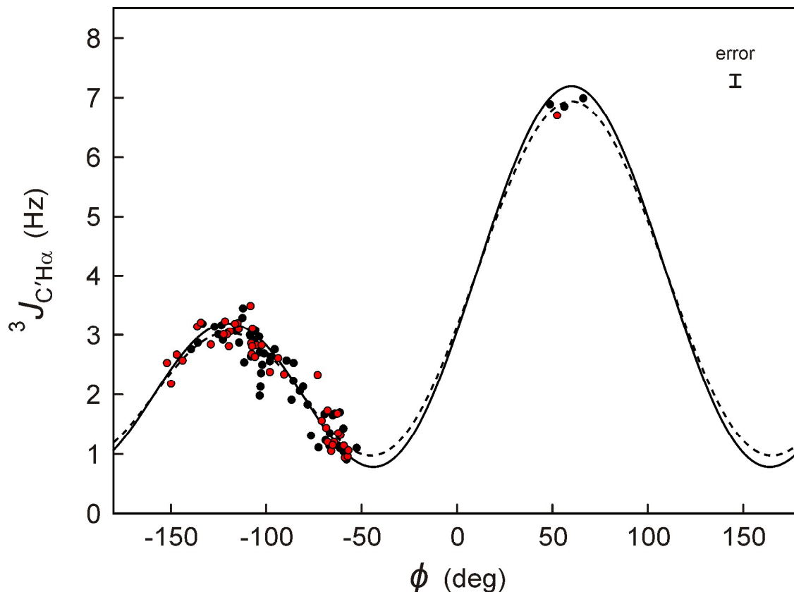
Fig. 4 Plot of experimental {}^3J_{C'H\alpha} coupling values against the backbone torsion angle \phi , for ubiquitin (black symbols) and GB3 (red). The backbone \phi values are derived from RDC-refined structures of GB3 (PDB entry 2OED) and ubiquitin (PDB entry 2MJB), both obtained without {}^3J_{C'H\alpha} data. The superimposed best-fit Karplus equation, shown as a dashed curve, is given by {}^3J_{C'H\alpha} = 3.76 \times \cos^2(\phi-60^\circ) + 1.95 \times \cos(\phi-60^\circ) + 1.23 . After factoring out the effect of Gaussian \phi angle fluctuations ( \sigma = 0.226 ), 52,51 the rigid limit Karplus equations (solid line) is given by: {}^3J_{C'H\alpha} = 4.17 \times \cos^2(\phi-60^\circ) + 2.00 \times \cos(\phi-60^\circ) + 1.02 . Residues with elevated backbone dynamics (L12, D40, and G41 for GB3; T9-K11, D32-G35, G47, D52, and R72-G76 for ubiquitin) are excluded from the plot and the fitting process. The error bar (top right) corresponds to the random error ( \pm 1 standard deviation) based on the reproducibility of the {}^3J_{C'H\alpha} measurements. The considerably larger RMSD of 0.25 Hz relative to the best-fitted Karplus curve (dashed line) reflects the impact of factors other than \phi on the {}^3J_{C'H\alpha} value.
