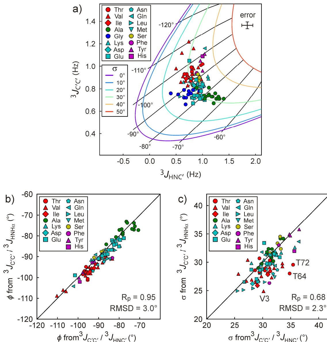
Fig. 7 Extracting the amplitude of \phi angle fluctuations from {}^3J_{C'C'} and {}^3J_{HNC'} . (a) Plot of {}^3J_{C'C'} versus {}^3J_{HNC'} for \alpha -synuclein. The rigid limit (after factoring out \sigma=13^\circ motions) {}^3J_{HNC'} Karplus parameterization 17 was used: {}^3J_{HNC'} = 4.78 \times \cos^2(\phi) + 0.86 \times \cos(\phi) - 0.23 Hz. Solid lines show correlations between {}^3J_{C'C'} and {}^3J_{HNC'} predicted by the dynamics-corrected Karplus equations for \phi angles ( \phi values marked by black “radial spokes”), with the different colors representing the amplitude of \sigma . The error bars (top right) corresponds to the random error ( \pm 1 standard deviation) of the {}^3J_{C'H\alpha} and {}^3J_{C'C'} measurements. (b) \phi and (c) \sigma values that are extracted from the {}^3J_{C'C'} and {}^3J_{HNC'} analysis are compared to those from {}^3J_{C'C'} and {}^3J_{HNC'} analysis, reported previously. 51
