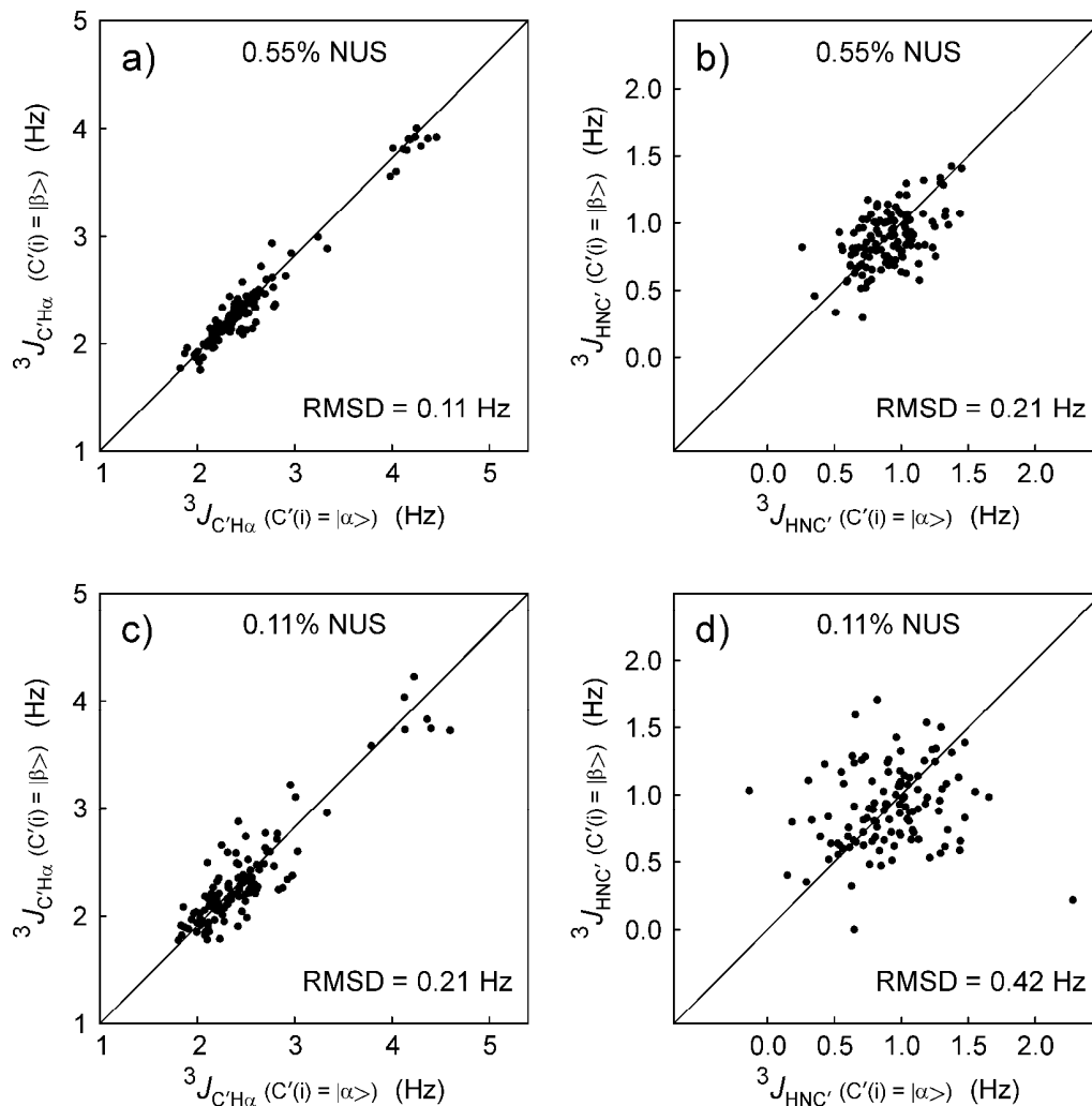
Fig. 3 Reproducibility of the duplicate measurements of ^3J couplings from the 4D NUS HACANH[C'] E.COSY spectrum of \alpha -synuclein. Comparisons of the duplicate ^3J_{C'Ha} measurements (see right panels of Fig. 2a) obtained when (a) using 0.55% NUS sampling and (c) 0.11% NUS sampling. Analogous comparisons of the two ^3J_{HNC'} measurements (see right two panels of Fig. 2c) obtained when using (b) 0.55% and (d) 0.11% NUS sampling.
