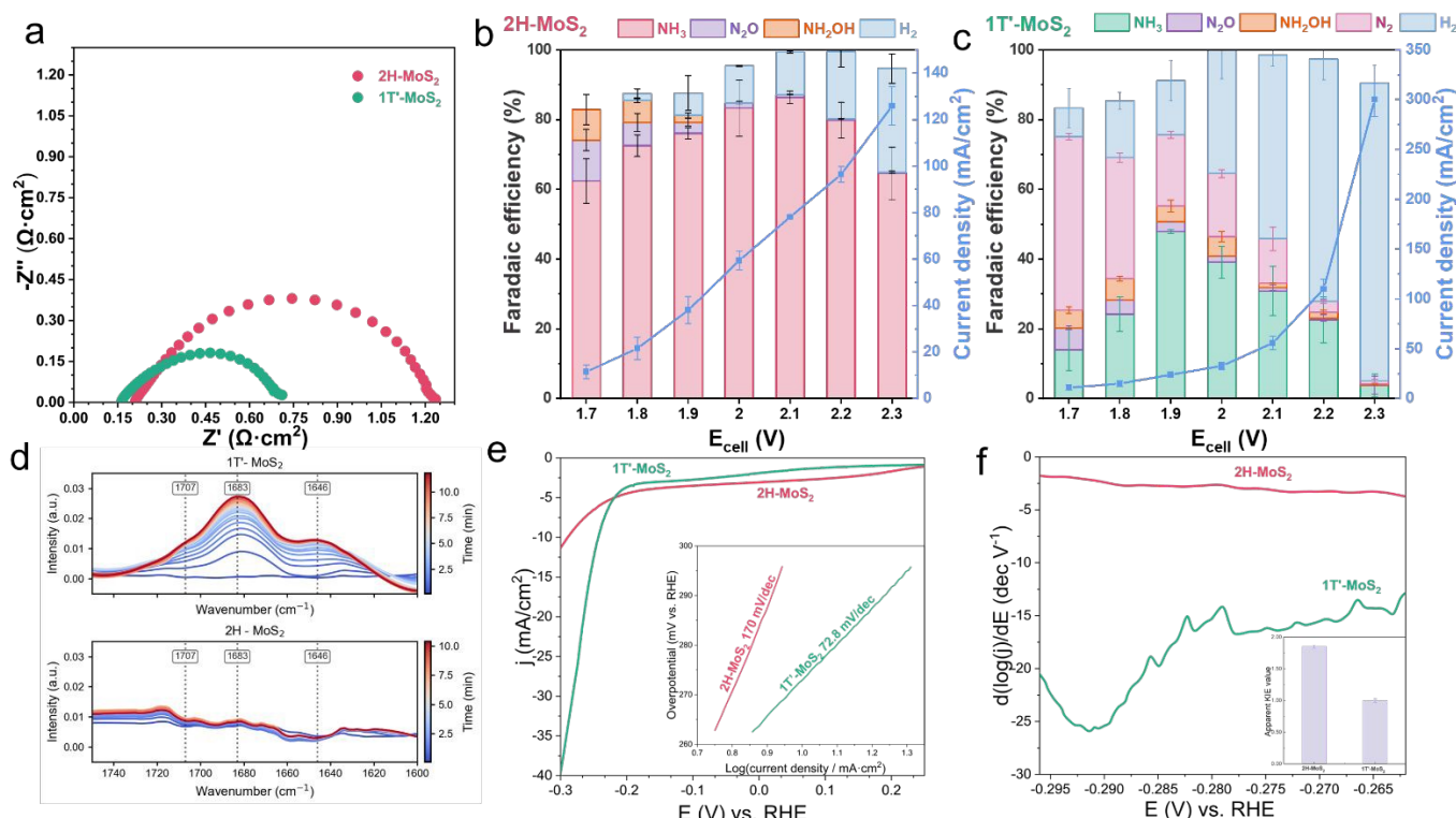
Figure 4. (a) EIS measurement for 2H and 1T' MoS 2 ; (b & c) faradaic efficiency and total current density for 2H and 1T' phase MoS 2 ; (d) NO adsorption for 2H and 1T' phase MoS 2 ; (e) LSV and Tafel slope; (f) local Tafel derivative and apparent KIE values for 2H and 1T' phase MoS 2 .
