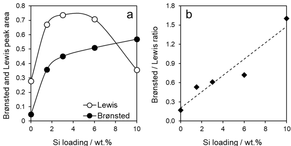
Fig. 5 Brønsted (1537 cm -1 ) and Lewis (1444 cm -1 ) acid sites peak area from pyridine/DRIFTS versus Si loading of the SiO 2 /ZrO 2 catalysts.
