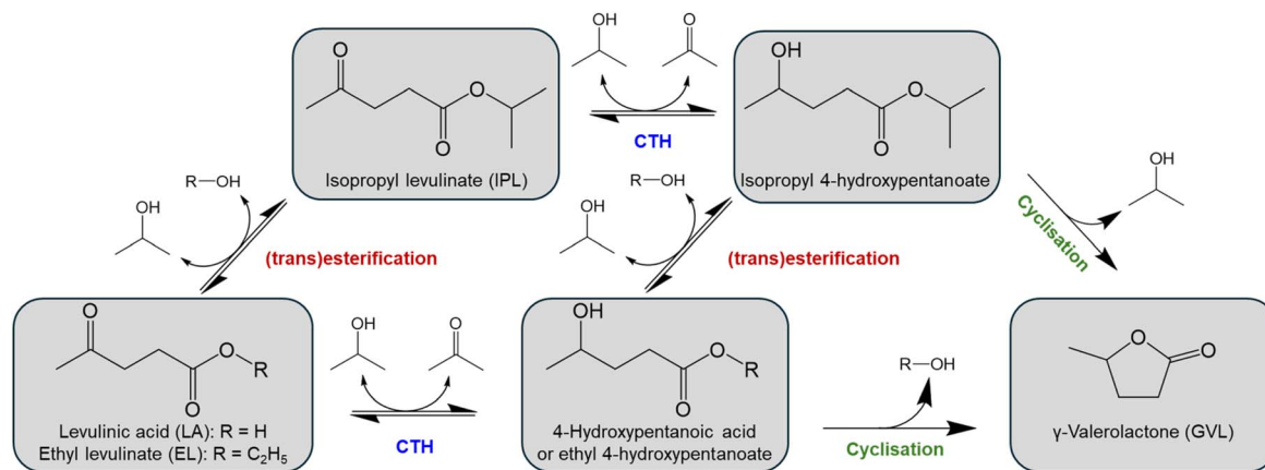
Fig. 8 The widely accepted reaction pathways for the liquid phase CTH of levulinic acid and ethyl levylate using 2-propanol as a hydrogen donor. 20,23,33,36
