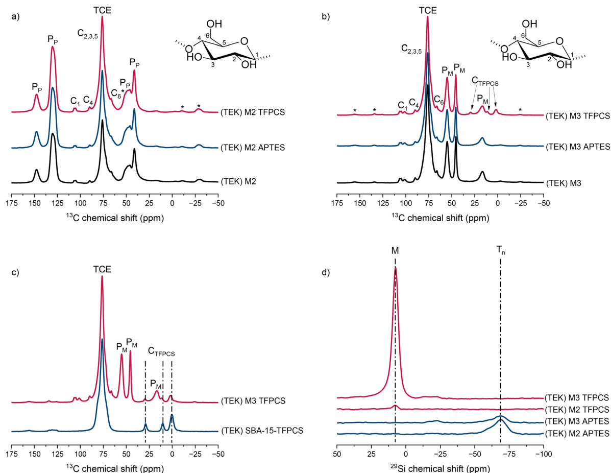
Fig. 6 (a) DNP-enhanced ^1\text{H} \rightarrow ^{13}\text{C} CP MAS spectra of the unmodified (linters paper + PS- b -PDHPMA membrane ( M2 )) and the APTES- and TFPCS-modified membranes. (b) DNP-enhanced ^1\text{H} \rightarrow ^{13}\text{C} CP MAS spectra of the unmodified membrane (linters paper + PMMA- b -PDHPMA membrane ( M3 )) and the APTES- and TFPCS-modified membranes. (c) DNP-enhanced ^1\text{H} \rightarrow ^{13}\text{C} CP MAS spectra of TFPCS-modified SBA-15 and TFPCS-modified membranes. (d) DNP-enhanced ^1\text{H} \rightarrow ^{29}\text{Si} CP MAS spectra of APTES- and TFPCS-modified membranes. Note: a 15 mM TEKPol in TCE (TEK) radical-solvent system was used for sample preparations. All spectra were recorded at a spinning rate of 8 kHz. Spinning sidebands are marked with an asterisk. Signals referring to the polymer are marked with "P".
