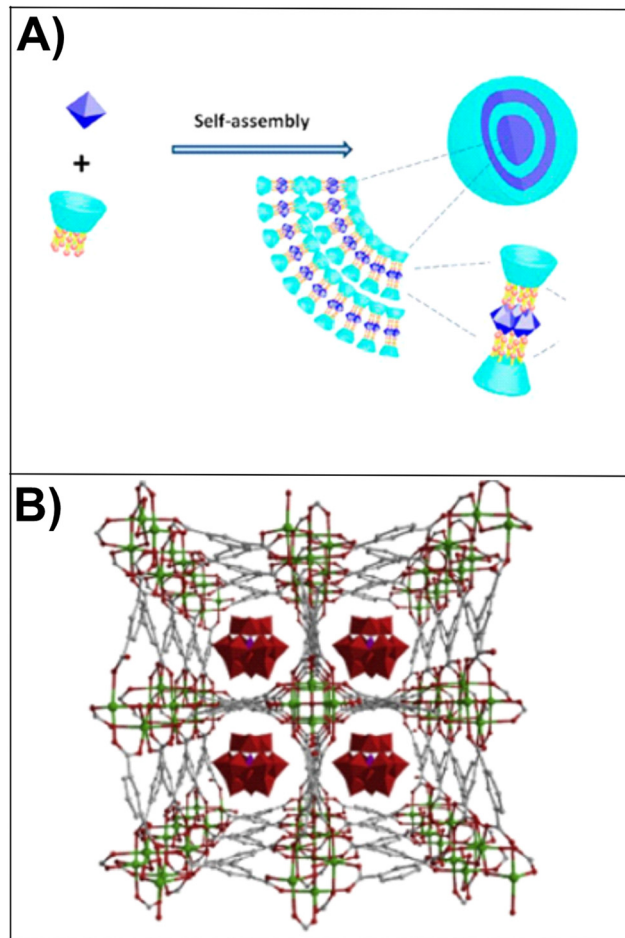
Fig. 13 A) Multivalent supramolecular self-assembly between β-cyclodextrin derivatives and polyoxometalate for photodegradation of dyes and antibiotics; reproduced from ref. 256 with permission from The American Chemical Society, copyright 2019. B) Encapsulate polyoxometalate into metal-organic frameworks as efficient and recyclable photocatalyst for drugs degradation; reproduced from ref. 257 with permission from Elsevier, copyright 2019.
