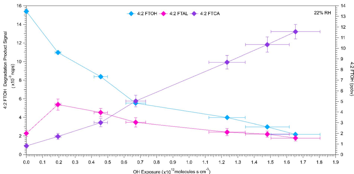
Fig. 2 The change in 4:2 FTOH (ppbv; m/z 265.027492) and the detected degradation products (4:2 FTAL, m/z 263.11842; 4:2 FTCA, m/z 279.006757; ncps) with increasing OH exposure (molecules s\ cm^{-3} ) at 22% RH. The right y-axis depicts the decreasing mixing ratio of permeating 4:2 FTOH, and the propagated error at each point, as it reacts with \cdot OH radicals. On the left y-axis are the normalized average signals of the degradation products, with each point's corresponding standard deviation. The x-axis shows the OH exposure and the propagated error at each point.
