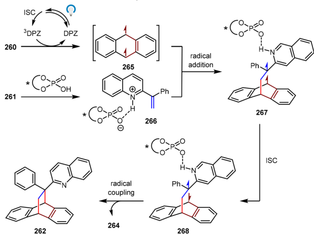
Scheme 53 Asymmetric [4+2] dearomatic photocycloadditions of anthracene with alkenylazaarenes.
