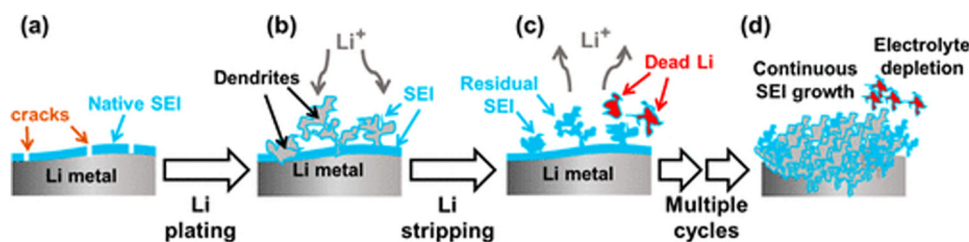
Fig. 9 Schematic diagram showing (from left to right) (a) pristine Li metal with heterogeneous native SEI layer, (b) growth of Li dendrites during Li plating, (c) loss of Li + (“dead Li”) and growth of residual SEI during Li stripping, and (d) continuous SEI growth and electrolyte depletion after multiple plating/stripping cycles. Reproduced under the terms of the ACS AuthorChoice License. 130 Copyright 2020, American Chemical Society.
