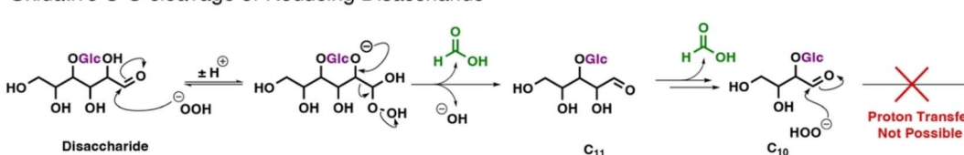
Scheme 3 Plausible mechanisms in the degradation of cellobiose in the presence of a hydroperoxyl anion. The absence of C 10 disaccharide and the rapid and full conversion to formate argue for a central role of Baeyer–Villiger oxidation.
