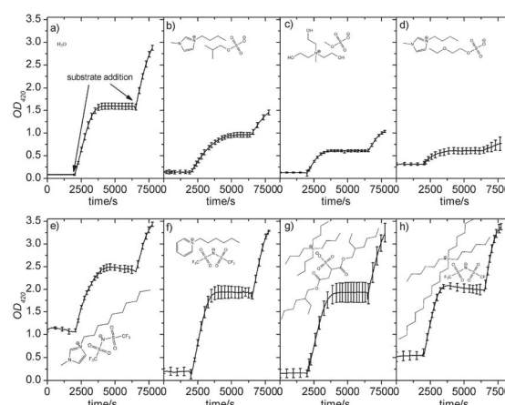
Fig. 8 Time course of laccase-catalysed ABTS oxidation in the presence of ILs. 96 (a) Control. (b) [\text{C}_4\text{mim}][\text{C}_3(2-\text{C}_1)\text{OSO}_3] , (c) [\text{N}_{1,2}(\text{OH})_3][\text{C}_1\text{OSO}_3] , (d) [\text{C}_4\text{mim}][\text{C}_2\text{OC}_2\text{OSO}_3] , (e) [\text{C}_{10}\text{mim}][\text{NTf}_2] , (f) [\text{C}_6\text{py}][\text{NTf}_2] , (g) [\text{N}_{4,4,4,4}][\text{AOT}] , and (h) [\text{P}_{6,6,6,14}][\text{NTf}_2] . (b), (c), and (d) are aqueous buffer (pH 4.5) solutions of the water-miscible ILs (20% (v/v)). (e), (f), and (g) are biphasic mixtures of buffer (pH 4.5) with water-immiscible ILs (20% (v/v)). Copyright RSC, 2012.
