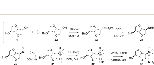
Fig. 20 Example of synthesis of CILs from isosorbide endo -mono-benzoate. 53
