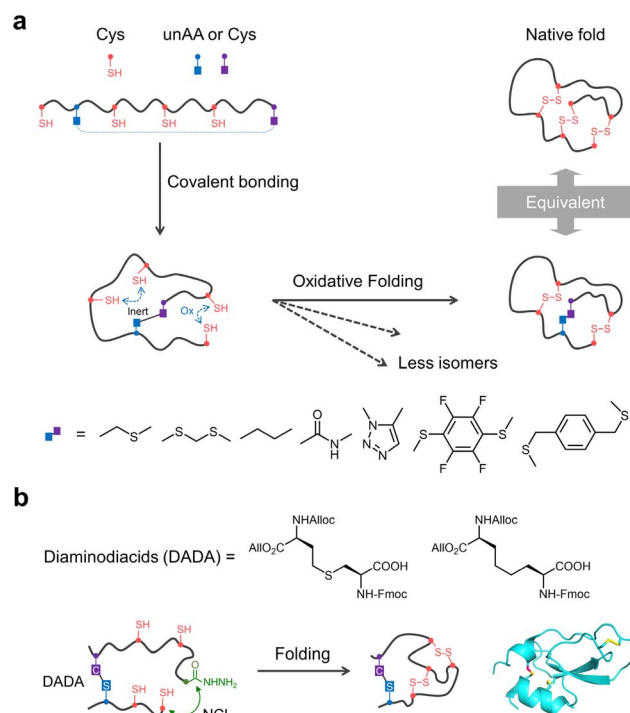
Fig. 3 (a) Oxidative folding of DRPs with non-reducible disulfide mimetics. unAA: unnatural amino acid; Ox: oxidation. (b) DRPs with cystathionine surrogates synthesized by NCL-assisted DADA approach and their structures (PDB ID: 6KZF).
