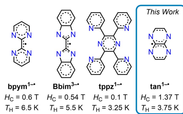
Fig. 1 Selected radical ligands used to construct dinuclear dysprosium single-molecule magnets [(Cp* 2 Dy) 2 (μ-L)]X with coercive fields ( H C ) and open magnetic hysteresis loops at or below this temperature ( T H ) under conventional sweep rates. Ligands L are: bpym = 2,2'-bipyrimidine (X = BPh 4 - ), Bbim = 2,2'-bisbenzimidazole (X = [K(crypt-222)] + , crypt-222 = 2.2.2-cryptand), tppz = 2,3,5,6-tetra(2-pyridyl)pyrazine (X = BPh 4 - ), tan = 1,4,5,8-tetraazanaphthalene (X = BArF 20 - ).
