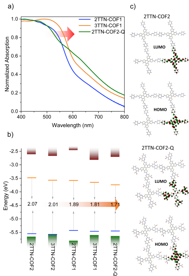
Fig. 3 (a) Diffuse reflectance spectra of the COF powders. (b) DFT-calculated (B3LYP/6-31G(d), red and green rectangles) and experimental (blue lines: PESA; orange lines: PESA + optical band gap) electronic levels of the COFs, and (c) DFT calculated orbital topologies for 2TTN-COF2 (top) and 2TTN-COF2-Q (bottom).
