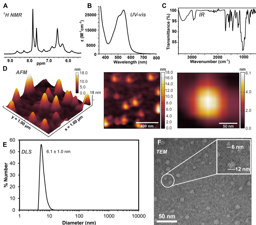
Fig. 3 Characterization data of [3][\text{BF}_4]_8 : (A) ^1\text{H} NMR spectrum ( \text{D}_2\text{O} , 45\text{ }^\circ\text{C} ); (B) UV-vis spectrum ( \text{H}_2\text{O} , 50\text{ }\mu\text{M} ); (C) ATR-IR spectrum; (D) AFM images and height profiles (tapping mode, air, 298\text{ K} ) of a drop-cast \text{H}_2\text{O} solution ( 0.2\text{ }\mu\text{M} ) on mica; (E) DLS measurement ( 50\text{ }\mu\text{M} , 85\% v/v DMSO/ \text{H}_2\text{O} ); (F) negative-contrast electron micrograph (uranyl acetate).
