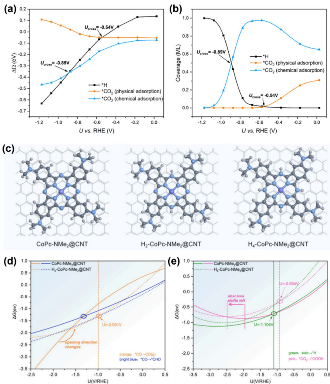
Fig. 9 (a) Potential-dependent reaction energetics of physical and chemical adsorption of \text{CO}_2 and \text{*H} formation on CoPc. (b) Potential-dependent competition of coverages among physical and chemical adsorption of \text{CO}_2 and \text{*H} formation on CoPc. 105 (c) Structural illustration of CoPc-NMe 2 @CNT, H 2 -CoPc-NMe 2 @CNT and H 4 -CoPc-NMe 2 @CNT. (d) and (e) Curves of Gibbs free energy change ( \Delta G ) for the key steps determining the potential for maximum MeOH selectivity for CoPc-NMe 2 @CNT, H 2 -CoPc-NMe 2 @CNT and H 4 -CoPc-NMe 2 @CNT as a function of applied potential. 106 Reproduced from ref. 105 and 106 with permission from American Chemical Society, copyright 2023, 2024.
