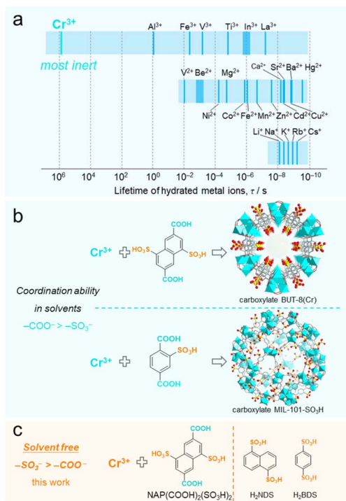
Fig. 1 Concept illustration of the solvent-free Cr- \text{SO}_3 coordination based on the inertness of the \text{Cr}^{3+} ion and the low coordination ability of the sulfonate group in the solvent. (a) Mean lifetimes of a water molecule ( \tau_{\text{H}_2\text{O}} ) in hydrated metal ions. 39–42 (b) The representative Cr-carboxylate BUT-8 and MIL-101- \text{SO}_3\text{H} with uncoordinated -\text{SO}_3\text{H}/-\text{SO}_3^- groups developed in solvents. 43,44 (c) Proposed coordination between the \text{Cr}^{3+} ion and the sulfonate group via solvent-free methods in this work.
