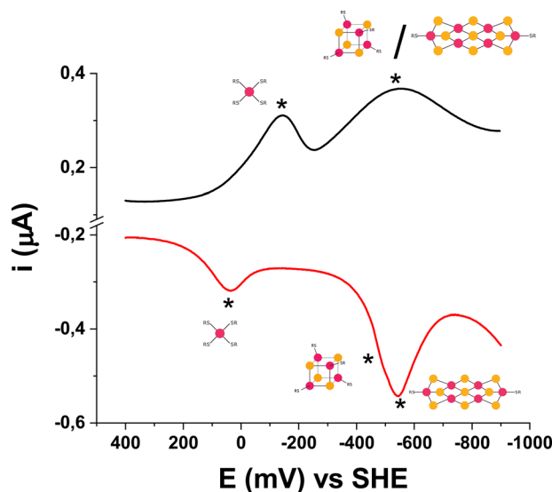
Fig. 2 Square wave voltammetry of 2:1 \text{HS}^-:\text{Fe}^{3+} glutathione (40 mM glutathione, 4 mM \text{Na}_2\text{S} , 2 mM \text{FeCl}_3 ) in \text{H}_2\text{O} , pH 8.6 and 20 °C. At this ratio, a well-defined anodic current peak is predominant at -0.55 \pm 0.01 V, together with traces of [\text{4Fe-4S}] (shoulder at -0.48 V). The peaks related to both the species are overlapped in the cathodic SW voltammogram (at -0.54 \text{ V} \pm 0.01 V). Peaks related to mononuclear complex ( -0.13 \pm 0.01 V and 0.04 \pm 0.01 V, cathodic and anodic peaks, respectively) are observed. The new species with E^\circ \sim -0.56 is tentatively assigned to a [\text{6Fe-9S}] cluster.
