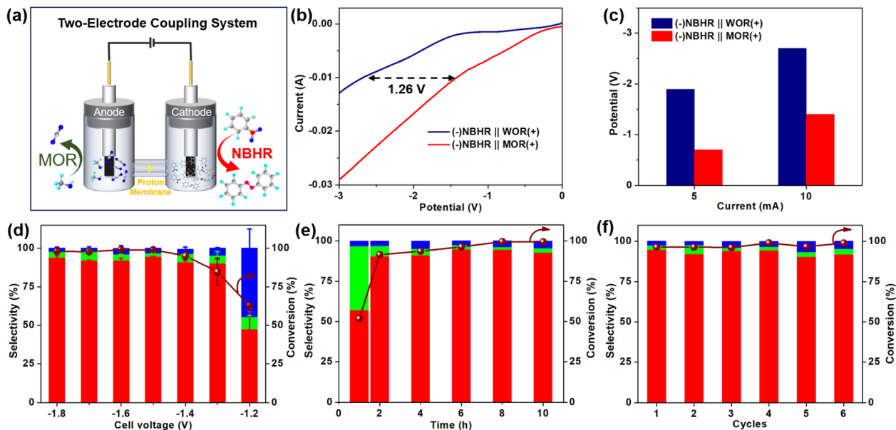
Fig. 5 Two-electrode coupling system. (a) A scheme illustrating the two-electrode coupling system with cathode NBHR and anode MOR. (b) LSV curves of PdS MNSSs in (-)NBHR||MOR(+) and (-)NBHR||WOR(+). (c) Cell voltages of PdS MNSSs at different current densities in (-)NBHR||MOR(+) and (-)NBHR||WOR(+). (d) Electrochemical selectivity and conversion of PdS MNSSs at different current densities in (-)NBHR||MOR(+). (e) Time-dependent electrochemical selectivity and conversion of PdS MNSSs in (-)NBHR||MOR(+) (-1.5 V). (f) Electrochemical stability of PdS MNSSs in (-)NBHR||MOR(+) (-1.5 V).
