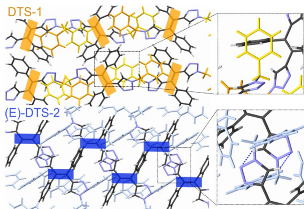
Fig. 3 Crystal structure of (E)-DTS-1 (top) and (E)-DTS-2 (bottom). Central double bonds are highlighted with a rectangle to show specific packing: herringbone (orange, (E)-DTS-1) and \beta -motif (blue, (E)-DTS-2). Zooms show specific intermolecular interactions: T-contacts in DTS-1 and triazole \pi -stacking in (E)-DTS-2.
