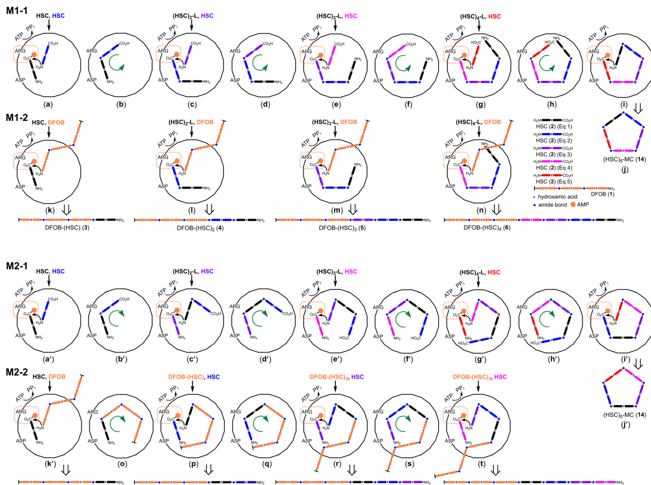
Scheme 3 Putative StDesD -mediated assembly of macrocyclic ( \text{HSC})_5\text{-MC} ( 14 ) by a processive mechanism with 2 predominating as the nucleophilic (M1-1: (a–j)) or carboxylate-activated (M2-1: (a'–j')) substrate. Putative assembly of \text{DFOB-(HSC)}_x ( x = 1\text{--}4 ) ( 3–6 , respectively) with 1 conserved as the nucleophilic substrate for condensation with pre-assembled carboxylate-activated 2 or 2 oligomers (M1-2: (k–n)), or 2 conserved as the carboxylate-activated substrate for condensation with 1 or 3–5 as pre-assembled nucleophilic substrates (M2-2: (k'–t)). Intracavity procession of intermediate substrates (green arrow) would enable the position of the carboxylic acid group of 2 or 2 oligomers is conserved for activation (broken orange box).
