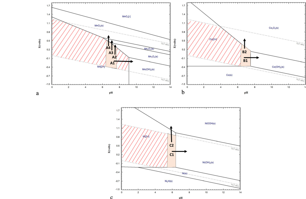
Fig. 3 Eh–pH diagrams for (a) Mn (1 mM), (b) Co (0.1 mM), and (c) Ni (0.1 mM), showing the predominant species in the H 2 O system at 25 °C.
