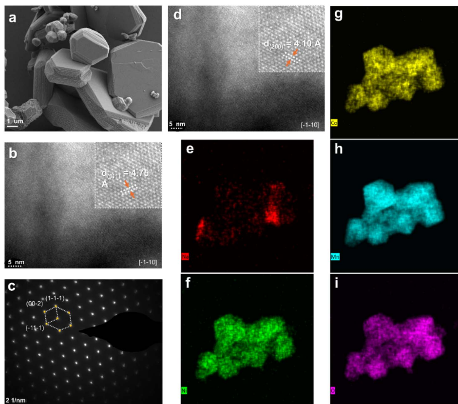
Fig. 3 Structural characterization of [NL]NCM material: (a) SEM (b–d) HRTEM image at the [-1-10] zone axis and the corresponding SAED image (e–i) TEM (HAADF Na, Ni, Co, Mn, and O) elemental mapping images of the [NL]NCM powder.
