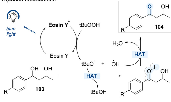
Scheme 57 Blue light-mediated chemoselective oxidation of 1,3-diol.
