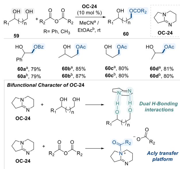
Scheme 34 DBN (OC-24) catalyzed regioselective acylation of diols.
