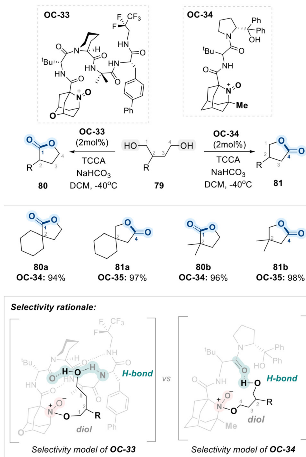
Scheme 45 Regiodivergent oxidation of unsymmetrical-1,4-enabled by OC-33 and OC-34 .
