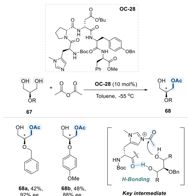
Scheme 39 Selective acylation of glycerol derivatives.
