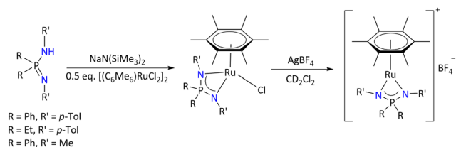
Scheme 28 Synthesis of the half-sandwich Ru(II) iminophosphonamide complex. 27
