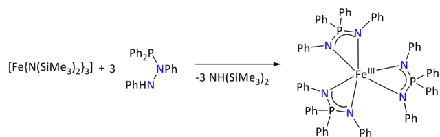
Scheme 27 Synthesis of the homoleptic Fe(III) iminophosphonamide complex. 93
