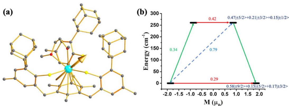
Fig. 10 (a) The g_{zz} axis of KD1 of complex [\text{U}(\text{OAr}^{\text{Ad, Me}})_3\text{mes}] ( 15 ). Colour code: U (cyan), S (yellow), O (red), C (grey). Hydrogens are omitted for clarity. (b) The mechanism of magnetisation relaxation of 8 . See Fig. 7 for more details in the figure caption.
