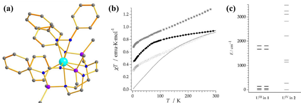
Fig. 16 (a) The molecular structure of the complex [(\text{SiMe}_2\text{NPh})_3\text{-tacn}]\text{U}(\eta^2\text{-N}_2\text{Ph}_2\text{C})] (27). (b) Colour code: U (cyan), N (blue), Si (violet), C (grey). Hydrogens are omitted for clarity. (b) A comparison of experimental and computed temperature-dependent magnetic susceptibility of 27 (experiment: grey squares for 27 and black circles for its precursor, computed: solid line). (c) The ground state energy splitting of 27 (right) and its precursor (left). Reprinted with permission from ref. 93 and reproduced with permission from John Wiley and Sons.
