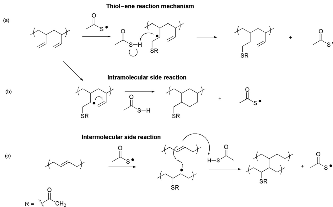
Fig. 4 (a) Thiol-ene click reaction mechanism, and (b and c) illustration of side reactions that account for a loss of double bonds and for an increase in polymer molecular weight and dispersity.
