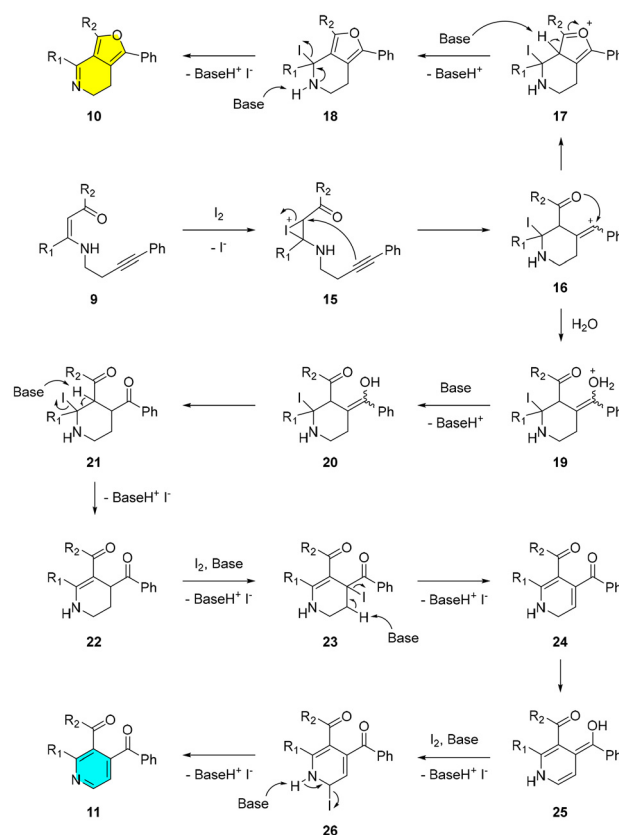
Scheme 7 Proposed mechanism for the formation of 6,7-dihydrofuro[3,4- c ]pyridines and 3,4-diarylpyridines.
