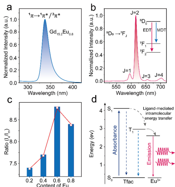
Fig. 2 (a) The excitation spectra of \text{Gd}_{15.2}\text{Eu}_{0.8} . (b) The emission spectra of \text{Gd}_{15.2}\text{Eu}_{0.8} . (c) Trend curve of I_e/I_{in} in different \text{Eu}^{3+} ratios. (d) Diagram of the energy transfer mechanism.
