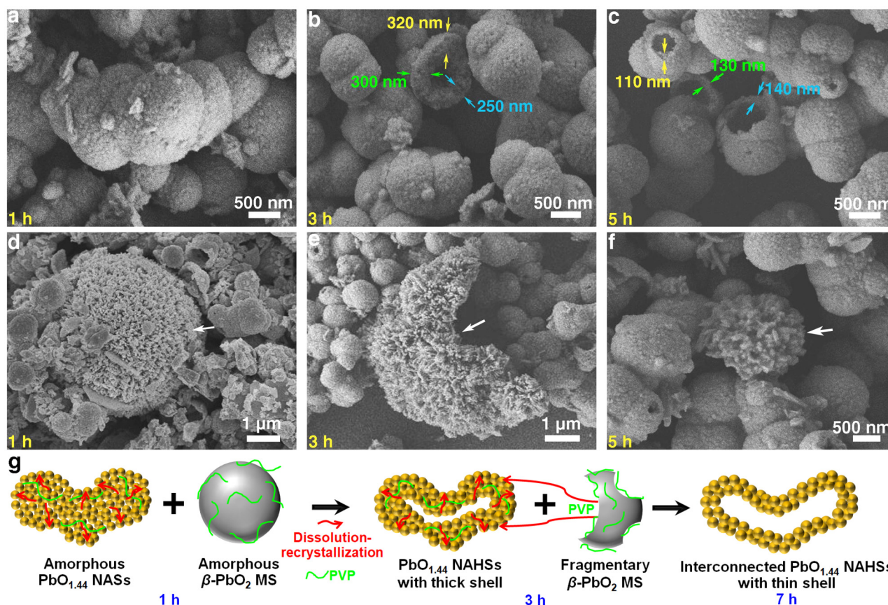
Fig. 4 Formation mechanism of \text{PbO}_{1.44} NAHSs. SEM images of representative intermediate particles of (a–c) \text{PbO}_{1.44} NAHSs and (d–f) \beta - \text{PbO}_2 MSs obtained after different reaction times of (a and d) 1, (b and e) 3 and (c and f) 5 h. (g) Schematic illustration of the formation mechanism of \text{PbO}_{1.44} NAHSs.
