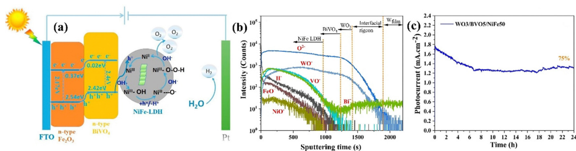
Fig. 19 (a) Schematic mechanism of PEC water splitting on Fe 2 O 3 /BiVO 4 /NiFe-LDH. Reproduced with permission from ref. 162, Copyright 2018, Elsevier. (b) TOF-SIMS profile of WO 3 /BiVO 4 /NiFe-LDH, (c) Stability test of the WO 3 /BiVO 4 /NiFe-LDH photoanode. Reprinted with permission from ref. 163, Copyright 2023, Elsevier.
