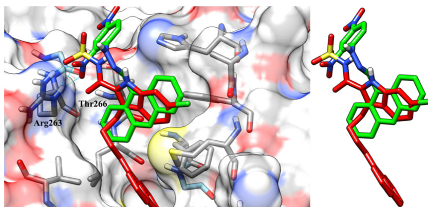
Fig. 16 Overlay of the docked molecule ( P1 green) and experimentally co-crystallized inhibitor (5WL red) within the binding domain of the Mcl-1 protein.
