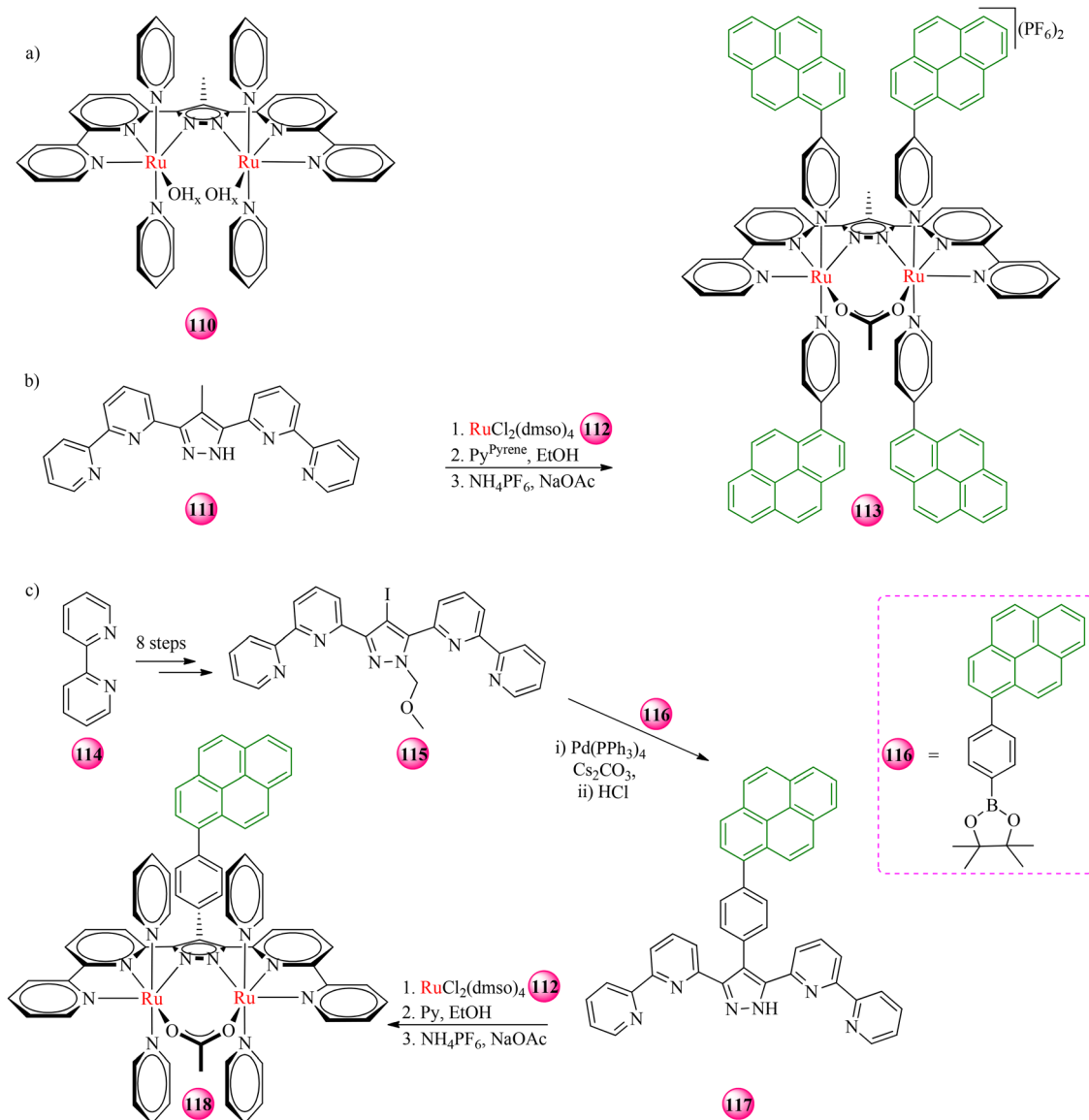
Fig. 36 (a) [(^{\text{Me}}\text{bbp})\text{Ru}(\text{OH})_2]_2(\text{py})_4 -type diruthenium WOC. (b) Synthesis of [(^{\text{Me}}\text{bbp})\text{Ru}_2(\text{OAc})(\text{py}^{\text{pyrene}})_4](\text{PF}_6)_2 ( 113 ). (c) Synthesis of ligand \text{pyrene}^{\text{bbpH}} with pyrene modification and complex [(^{\text{pyrene}}\text{bbp})\text{Ru}_2(\text{OAc})(\text{py})_4](\text{PF}_6)_2 ( 118 ). Reproduced with permission from ref. 53 copyright 2020, American Chemical Society.
