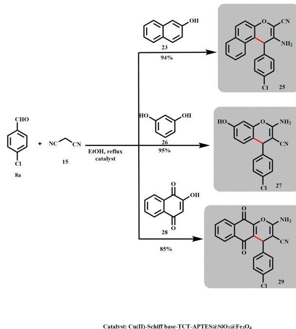
Scheme 12 Cu(II)-Schiff base-TCT-APTES@SiO 2 @Fe 3 O 4 catalysed synthesis of chromene derivatives (Kalantar et al. ).
