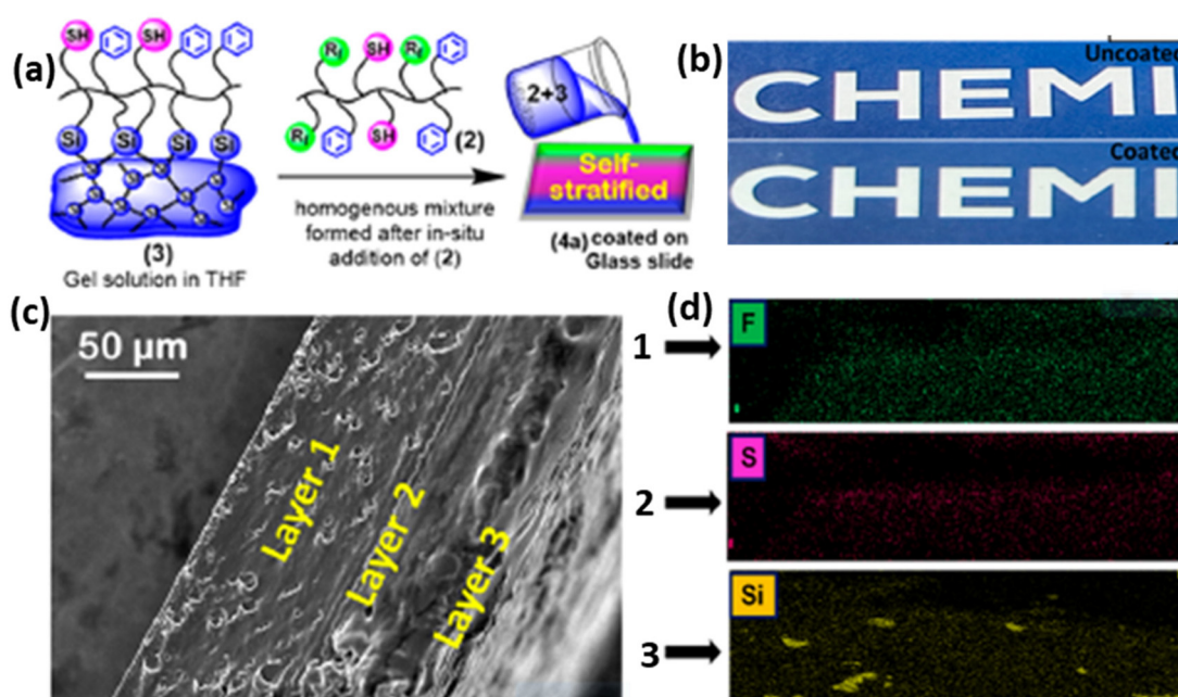
Fig. 15 (a) Graphical representation of the formation of self-stratified polymers based on fluorosulfonyl/thiol/siloxane, (b) comparison of uncoated and coated polymers on glass, (c) SEM images of a cross-section of the cured film, and (d) corresponding EDX dot mapping of three positions. Reproduced with permission; 97 Copyright 2023, ACS.
